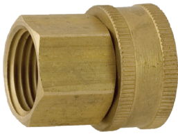
Brass 3/4" Female Hose x 1/2" Female Pipe Swivel
